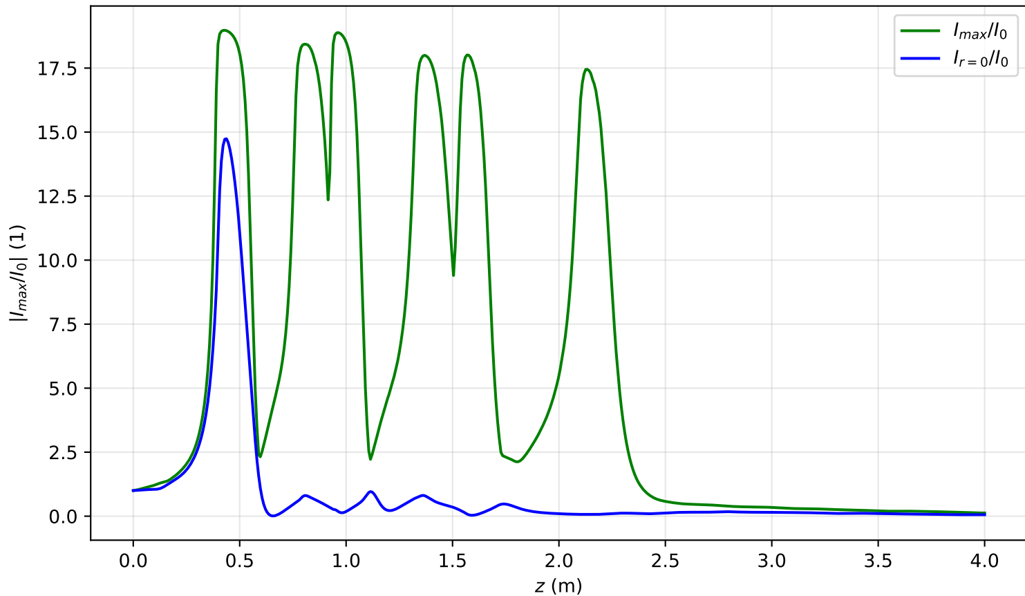
I_{max}(x = 0, y = 0, z)/I_0 , Pin=5.8P_{cr} , noisy input, artificial time
